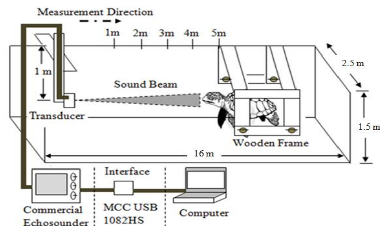
Fig. 2. The illustration of experiment setup
