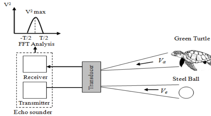
Fig. 1. Target strength measurements using a reference sphere
