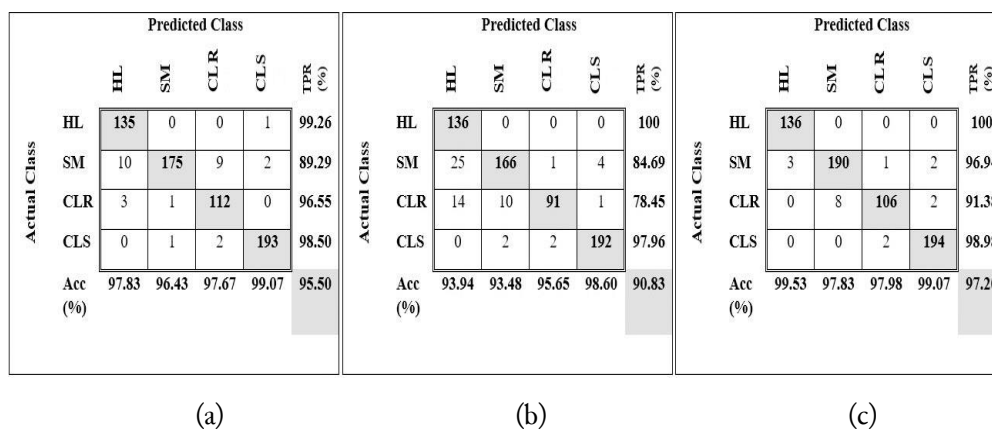
Fig. 8. Confusion Matrix: Xception (a), ResNetV2-152 (b), VGG16 (c)
